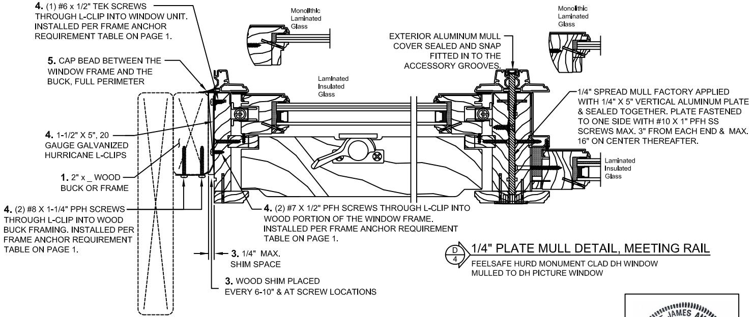
JAMB DETAIL FEELSFAE HURD MONUMENT CLAD DOUBLE HUNG WINDOW
